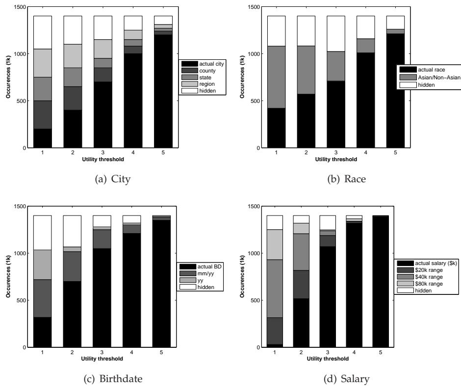
Figure 11: Effect of Utility Threshold on the Level of Attribute Disclosure
